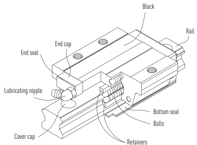
Fig. Construction of the HG series
