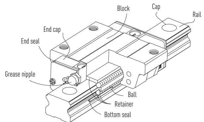
Fig. Construction of the EG series
