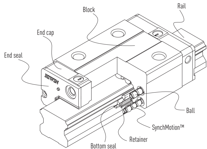
Construction of the QE series
