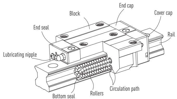
Fig. Construction of the RG series
