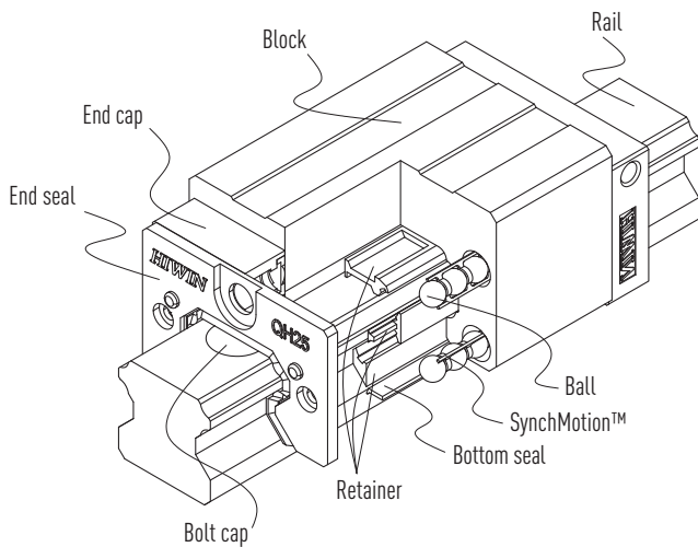
Construction of the QH series
