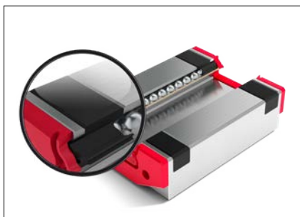
Enlargement of ball recirculation in the carriages
