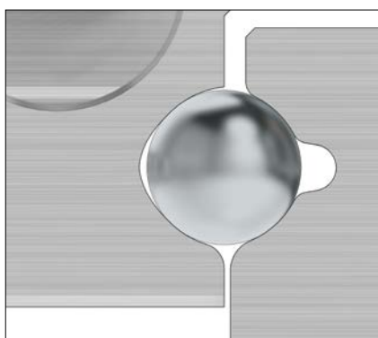
Gothic arc profile of the guideway tracks
