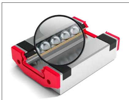
Retaining wire holding the balls in place
